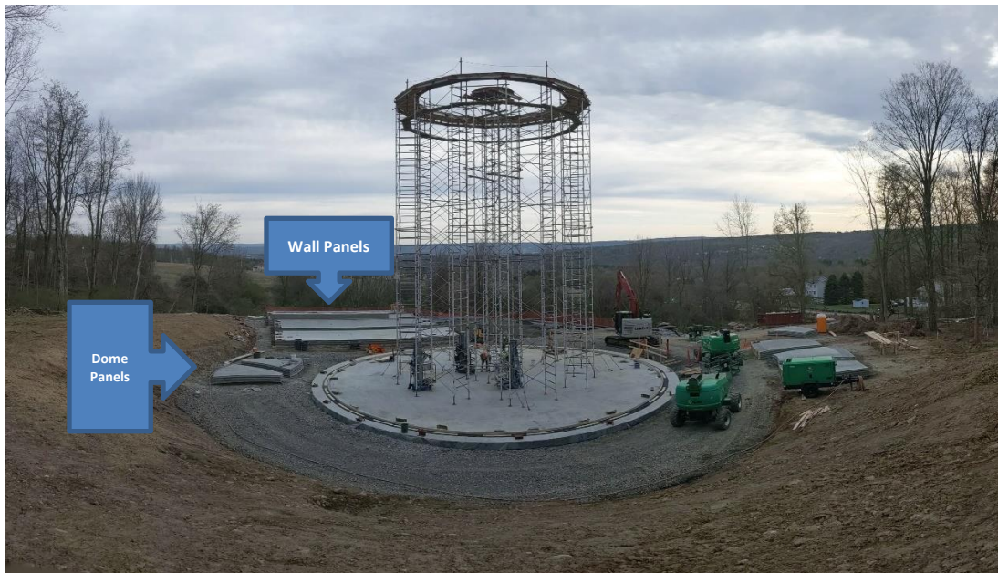
Erecting temporary support structure. Note pre-cast concrete panels for Roof Dome & Walls.
