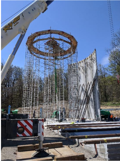
Erecting Precast Concrete & Steel Wall Panels. Note Panels in Foreground.
